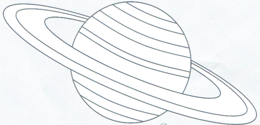
Saturn
